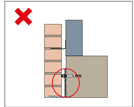
Non-plumb structure examples
