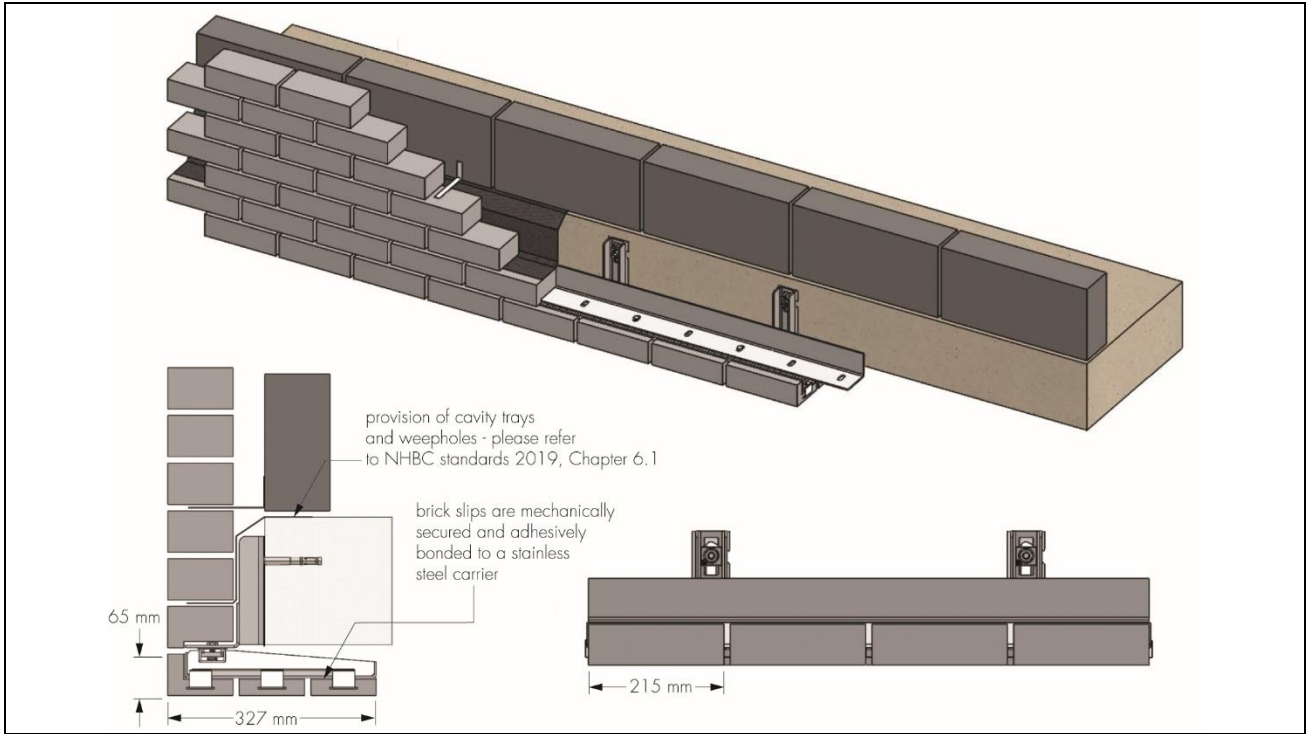
Figure 2 BOSS 65 x 327 mm with stretcher bond (welded masonry support, shims and anchor bolts are outside the scope of this Certificate)
