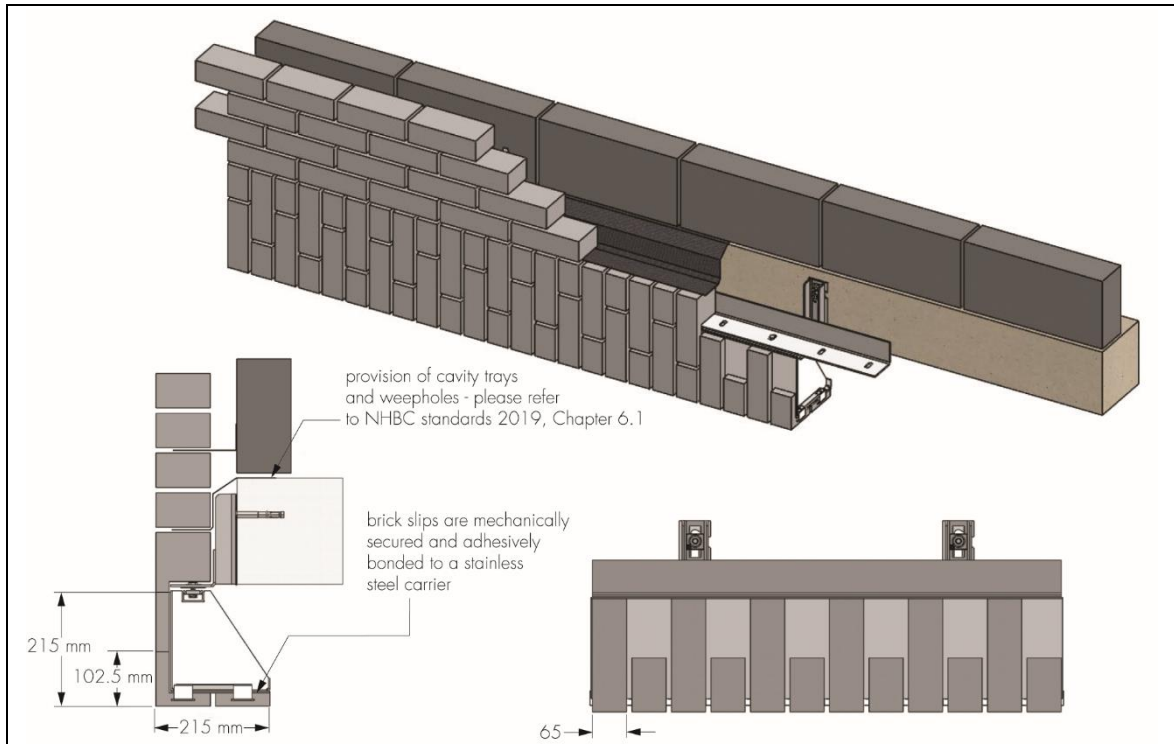
Figure 3 BOSS 215 x 215 mm with half lap bond (welded masonry support, shims and anchor bolts are outside the scope of this Certificate)
