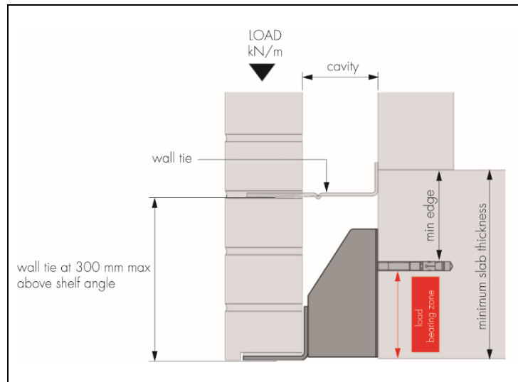
Figure 5 The IG Welded Masonry Support System
