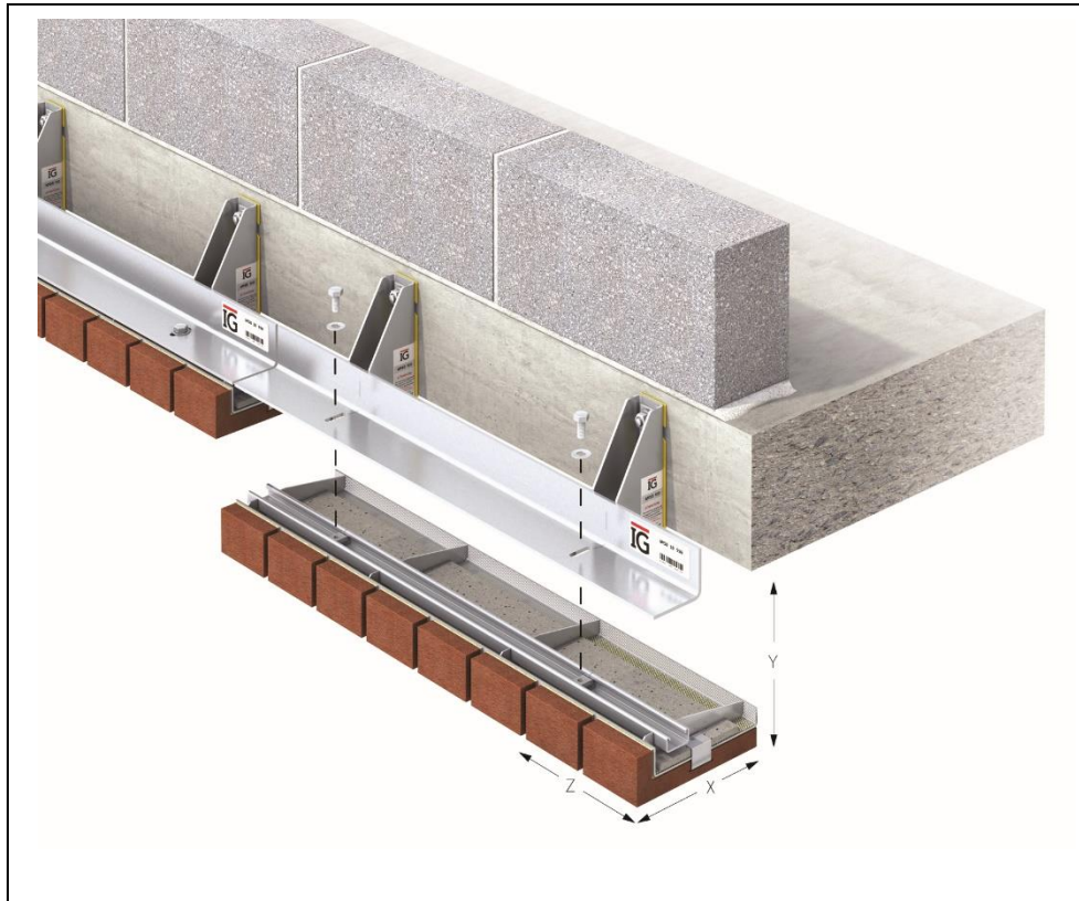
Figure 7 Adjustment of the IG Brick On Soffit System (B.O.S.S.+)
