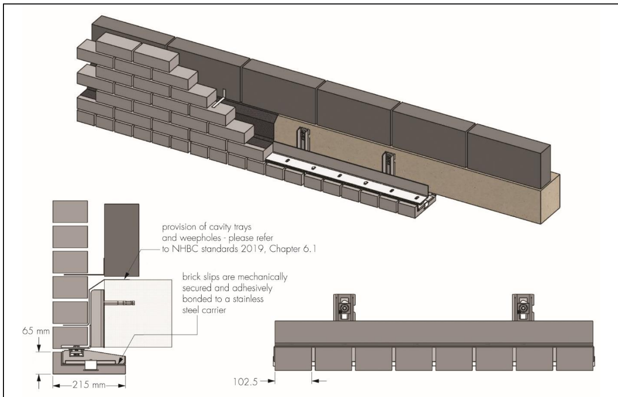
Figure 1 BOSS 65 x 215 mm with header bond (welded masonry support, shims and anchor bolts are outside the scope of this Certificate)
