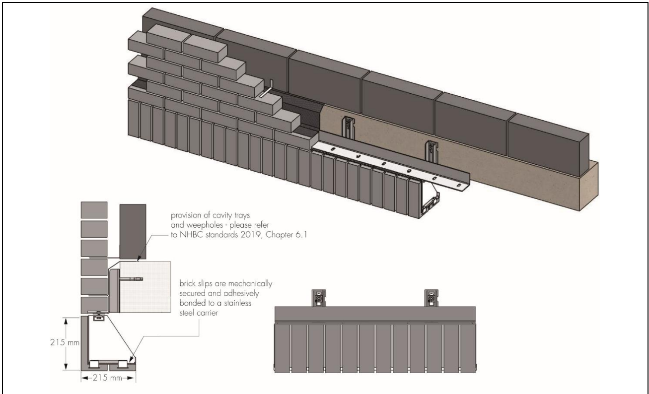
Figure 4 BOSS 215 x 215 mm with soldier bond (welded masonry support, shims and anchor bolts are outside the scope of this Certificate)
