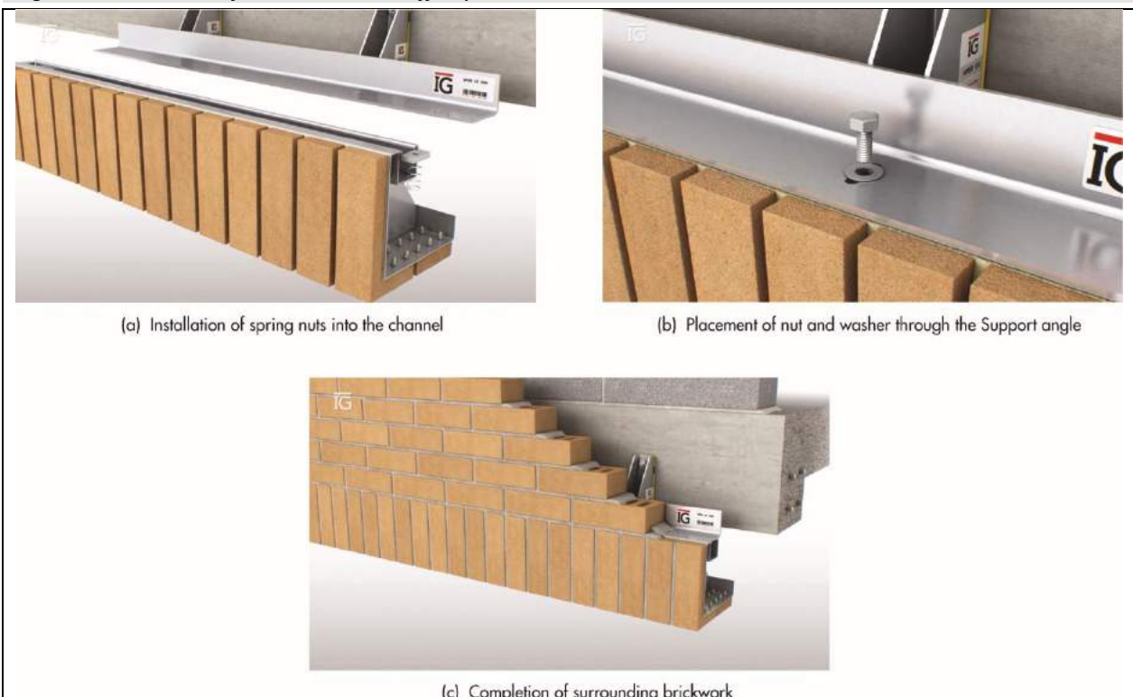
Figure 6 Installation of the IG Brick On Soffit System
