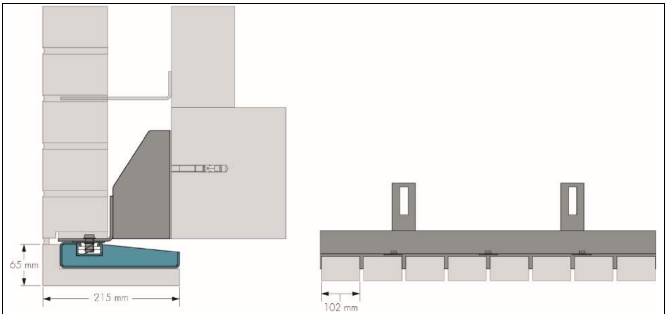
Figure 1 BOSS 65 x 215 mm with Header Bond (welded masonry support, shims and anchor bolts are outside the scope of this Certificate)
