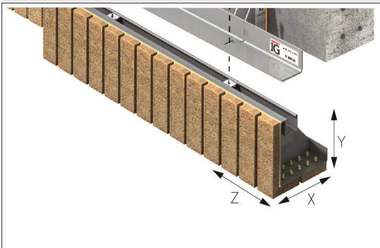
Figure 7 Adjustment of the IG Brick On Soffit System
