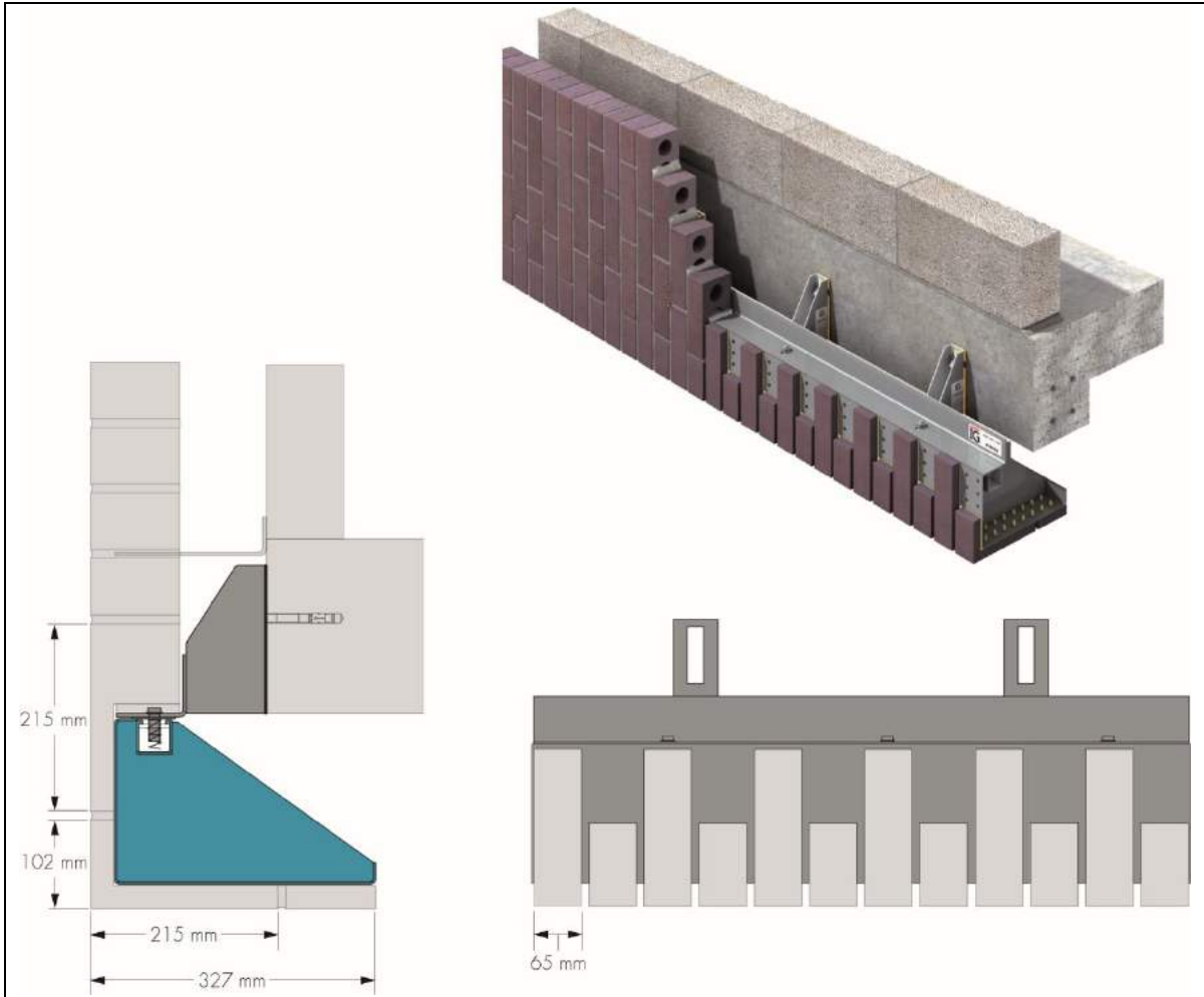
Figure 3 BOSS 215 x 327 mm with Half Lap Bond (welded masonry support, shims and anchor bolts are outside the scope of this Certificate)
