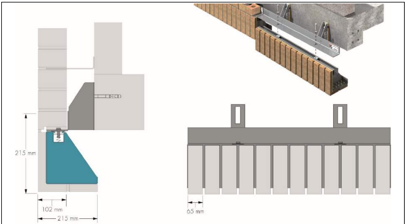
Figure 4 BOSS 215 x 215 mm with Soldier Bond (welded masonry support, shims and anchor bolts are outside the scope of this Certificate)
