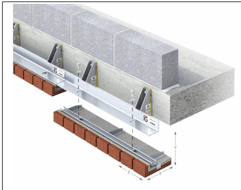
Figure 7 Adjustment of the IG Brick On Soffit System (B.O.S.S.A1)
