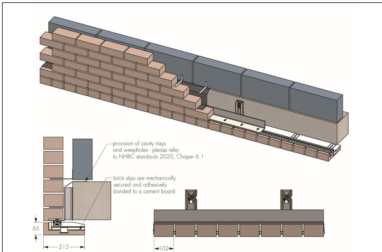
Figure 1 BOSS A1 65 x 215 mm with header bond (welded masonry support, shims and anchor bolts are outside the scope of this Certificate)
