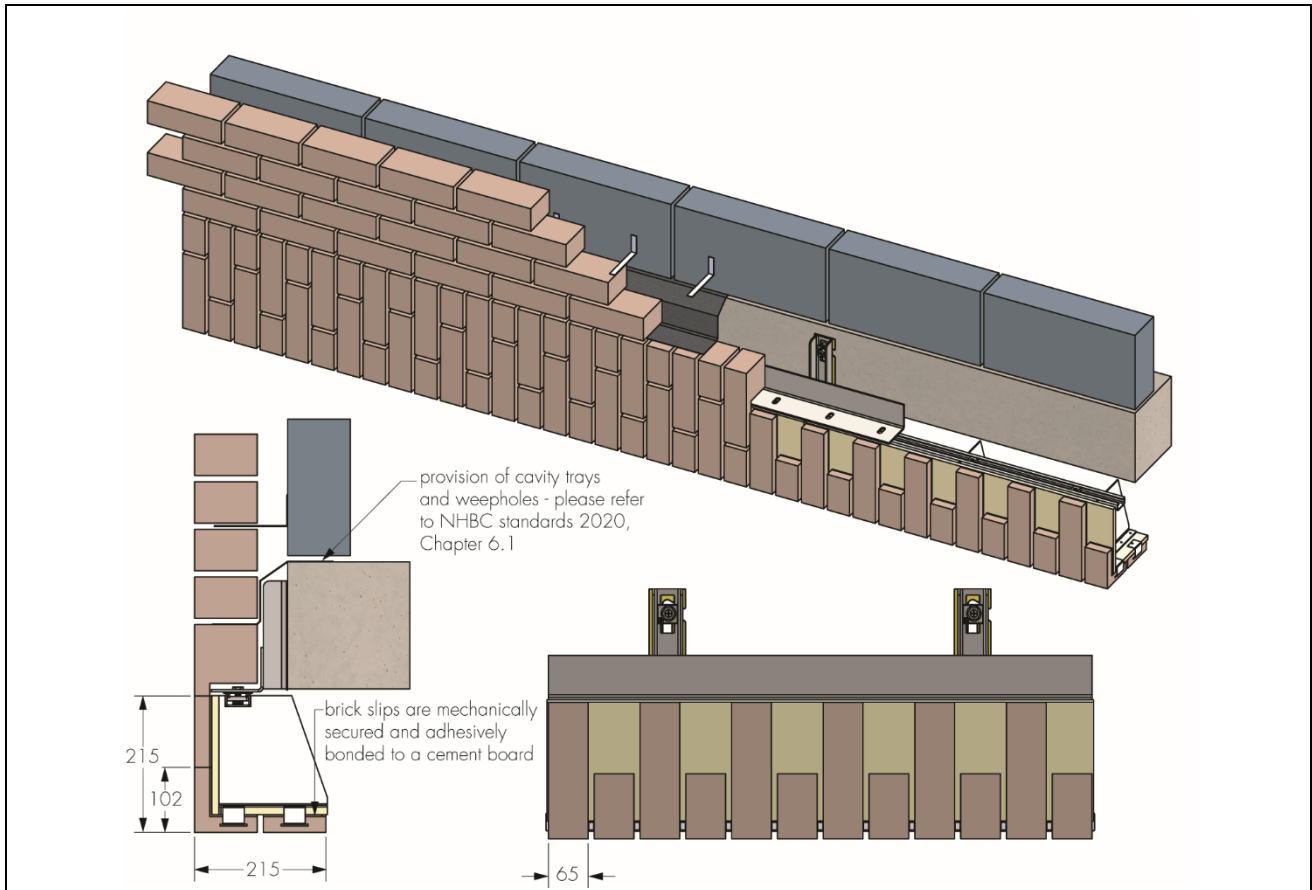
Figure 4 BOSS A1 215 x 215 mm with soldier bond (welded masonry support, shims and anchor bolts are outside the scope of this Certificate)
