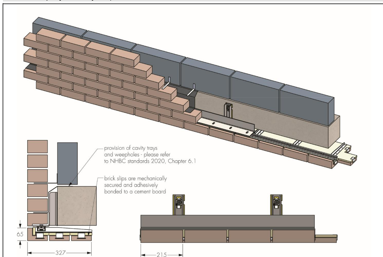
Figure 2 BOSS A1 65 x 327 mm with stretcher bond (welded masonry support, shims and anchor bolts are outside the scope of this Certificate)
