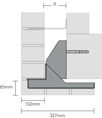
Stretcher 65-327
