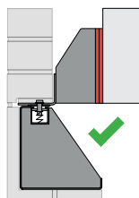
Maximum shimming not exceeded
